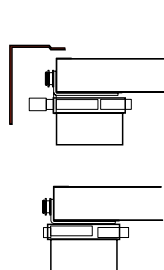
Burlete lateral
