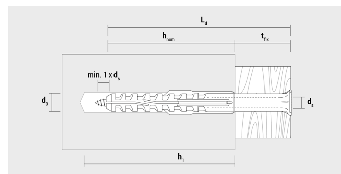
MFR 8: d_1 = 6 mm, MFR 10: d_1 = 7 mm, MFR 14: d_1 = 10 mm
